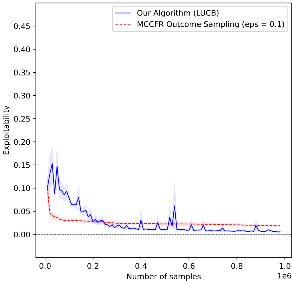
RBT, Start Policy, Player x
